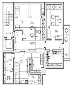
PLAN MOBILARE - CLINICA - MANSARDA
